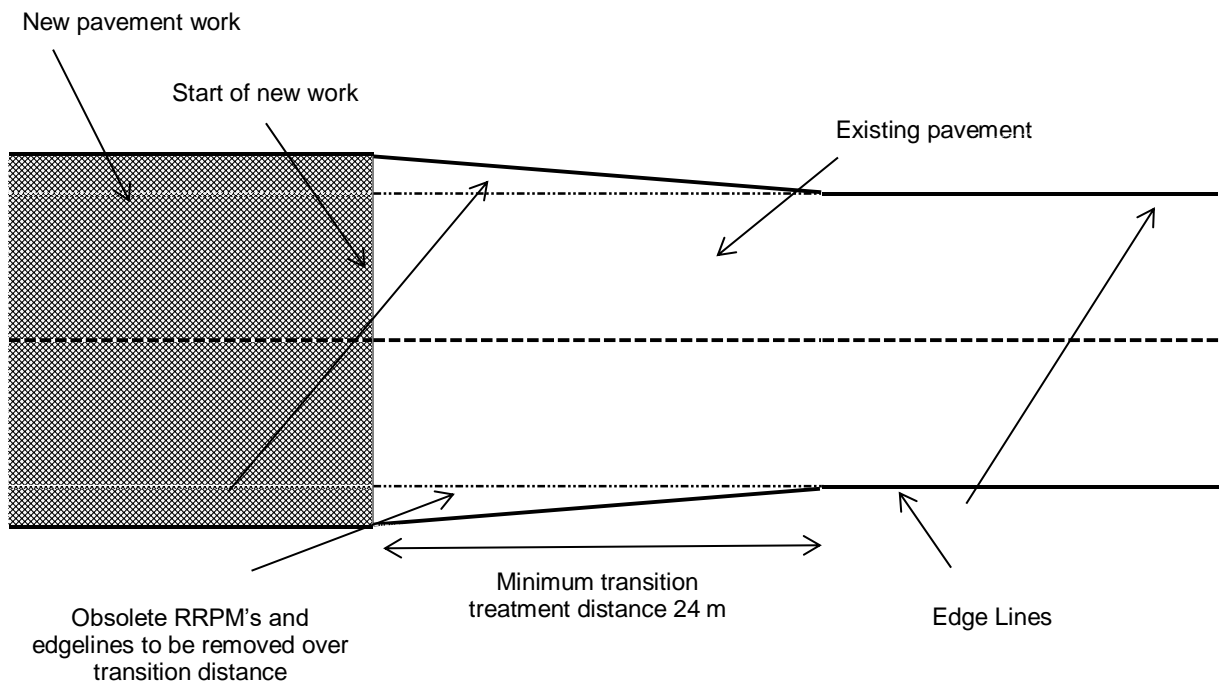
Figure 5.16 Edge line Mismatch Treatment
